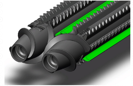
⊕ Dual cutting flutes provide improvements in stalk sizing.
