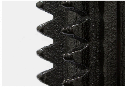
⊕ Specially designed teeth for crimping the stalk.
